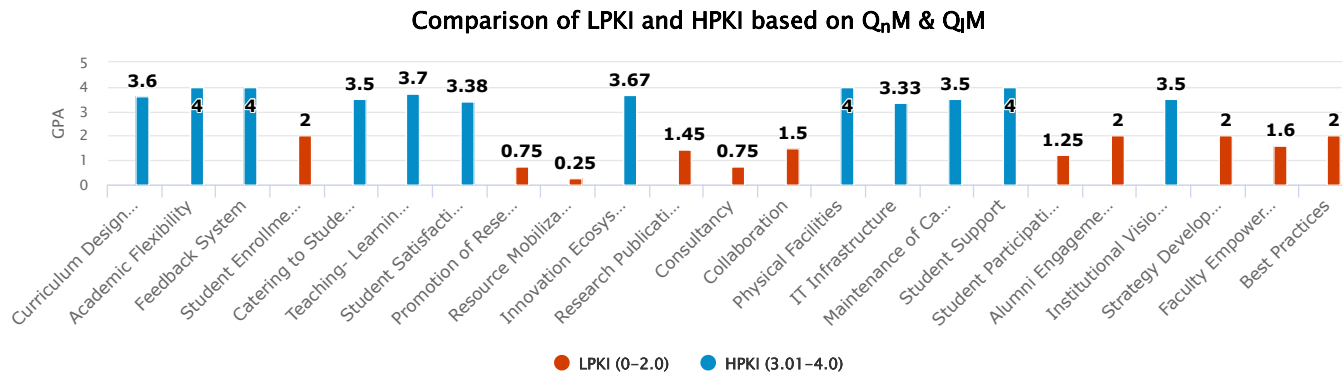
Fig: Comparison of LPKI(0-2.0) and HPKI(3.01-4.0) based on Q n M & Q 1 M
